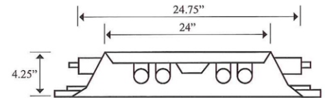
Type M Mechanical or Plaster Ceiling Plaster Frames (Optional)
